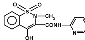
Figure 1. Structure of piroxicam.
